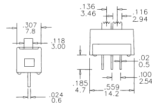
CT Series top actuator
