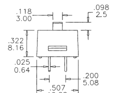
Double pole
