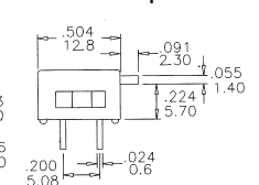
Double pole
