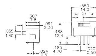
CT Series side actuator
